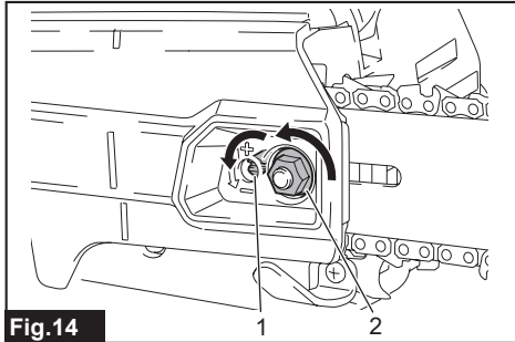
Fig. 14 ▶ 1. Chain adjusting screw 2. Retaining nut
