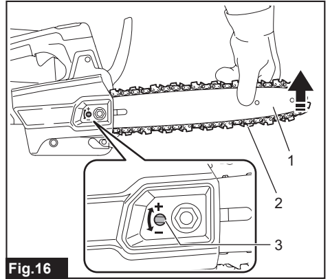
Fig. 16 ▶ 1. Guide bar 2. Saw chain 3. Chain adjusting screw
